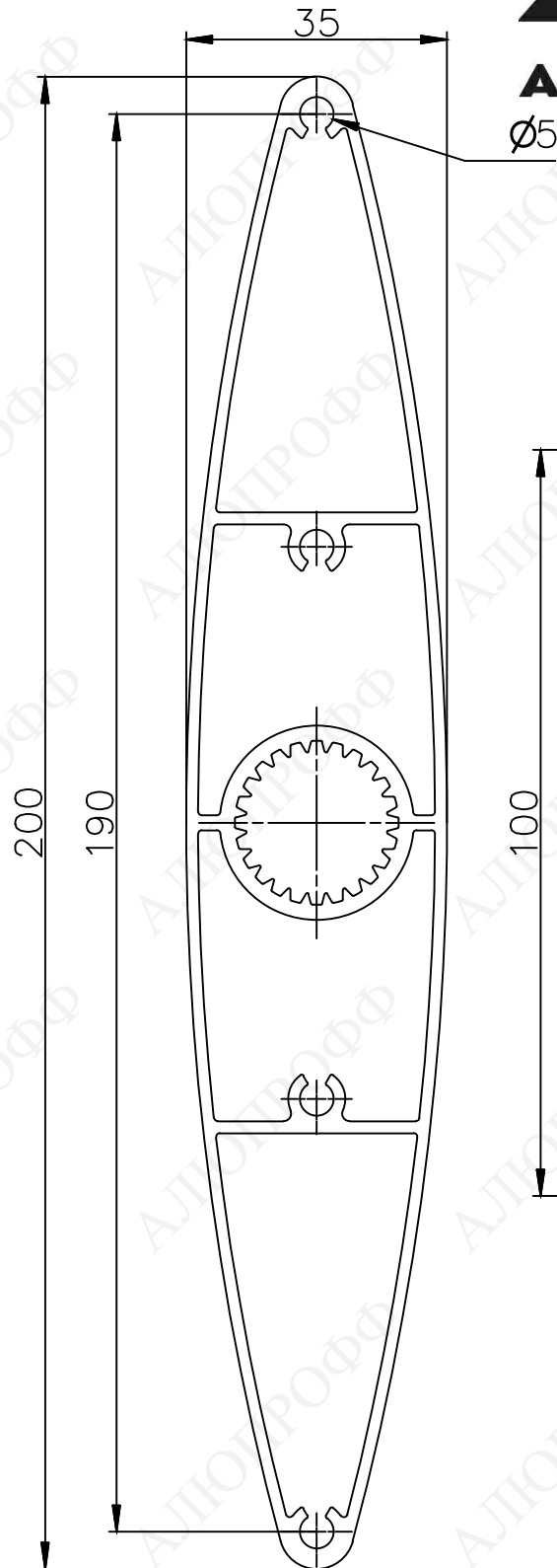
ALW200
