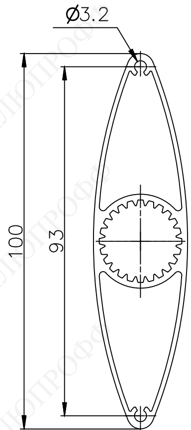
ALW100
